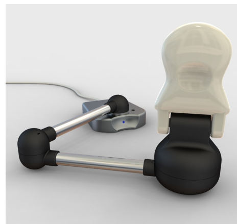
Figure 1: Planar constrained surface controller
